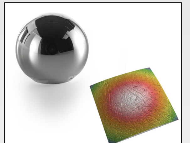
Quality control of a cobalt-chromium polished prosthesis surface (DHM S2)
