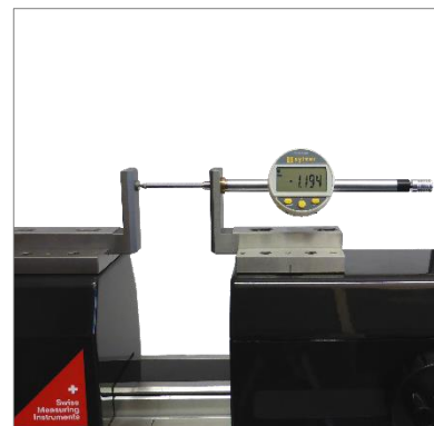
Checking of dial indicator (TEL5CN)
