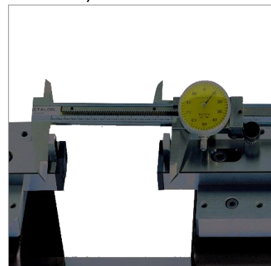
Checking of calipers (TEL 5.10)
